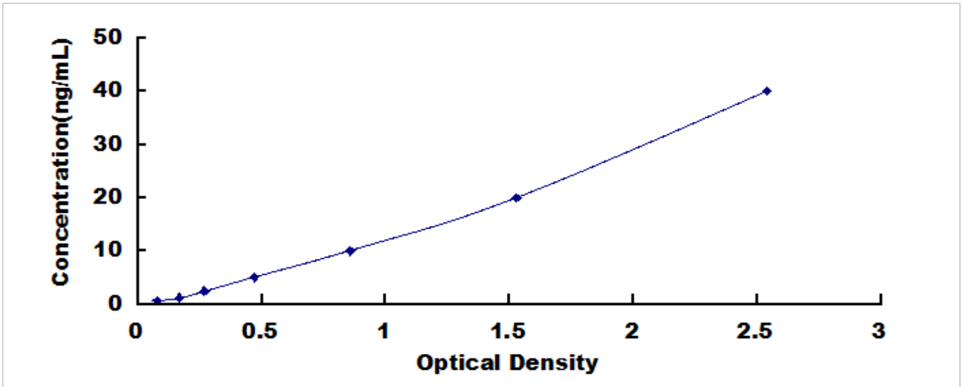
Typical Standard Curve for GAL1, Rat ELISA.
