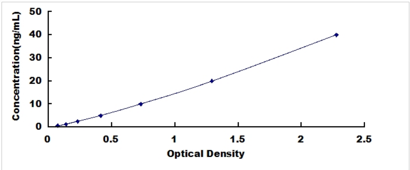
Typical Standard Curve for GAL1, Rat ELISA.
