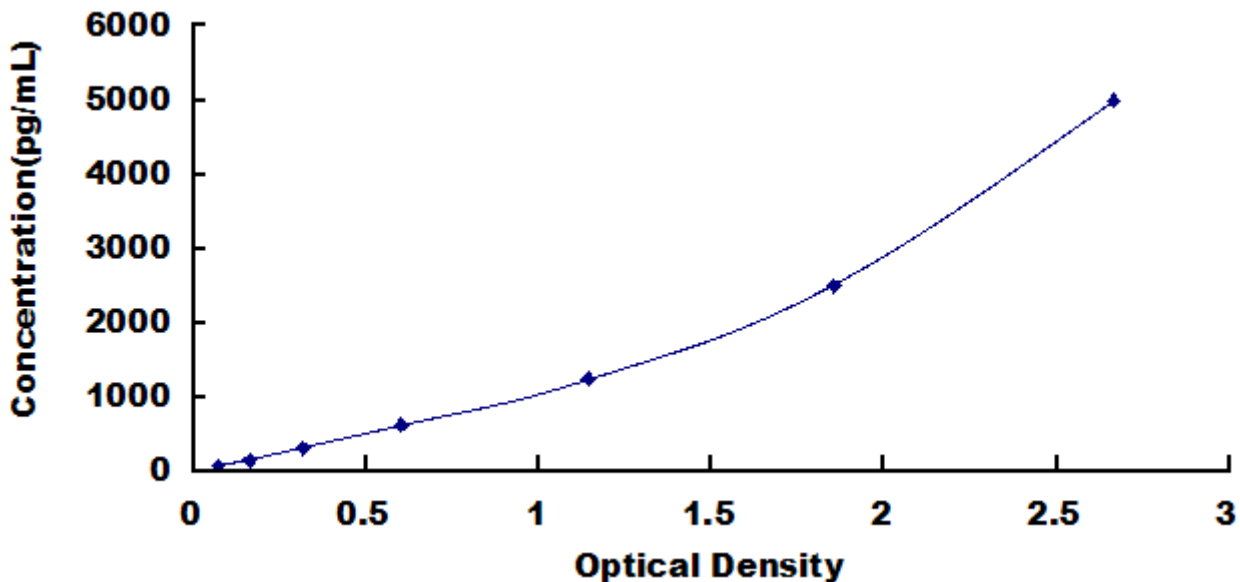
Typical Standard Curve for GLUT2, Human ELISA.
