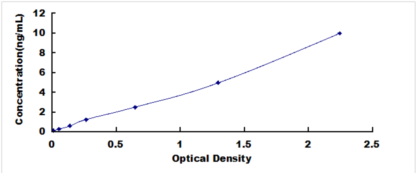
Typical Standard Curve for AGL, Human ELISA.
