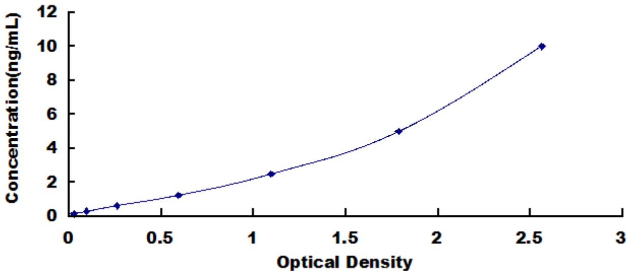
Typical Standard Curve for HIP2, Human ELISA.
