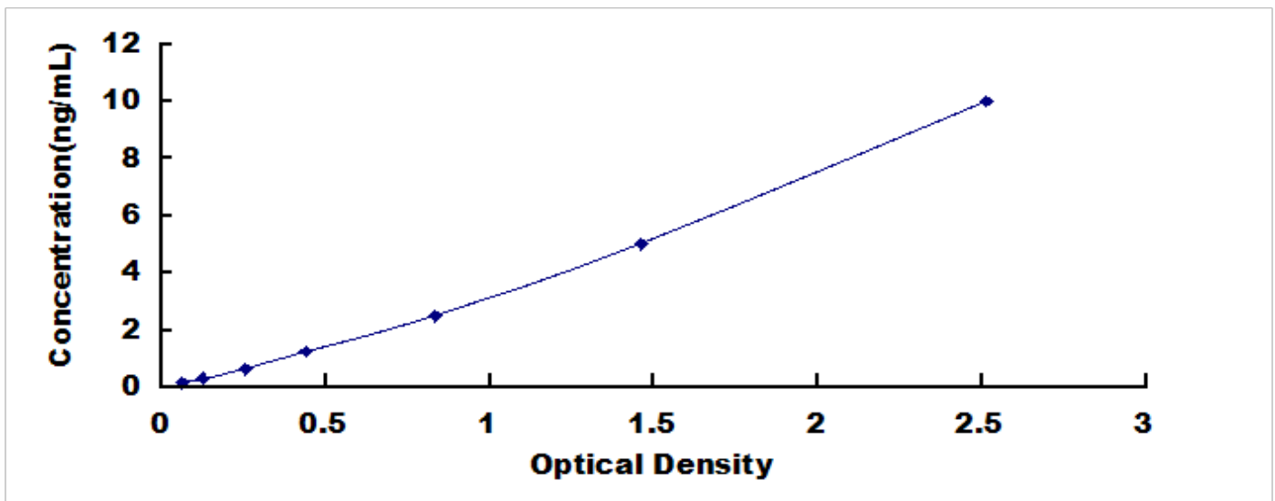
Typical Standard Curve for IDE, Mouse ELISA.
