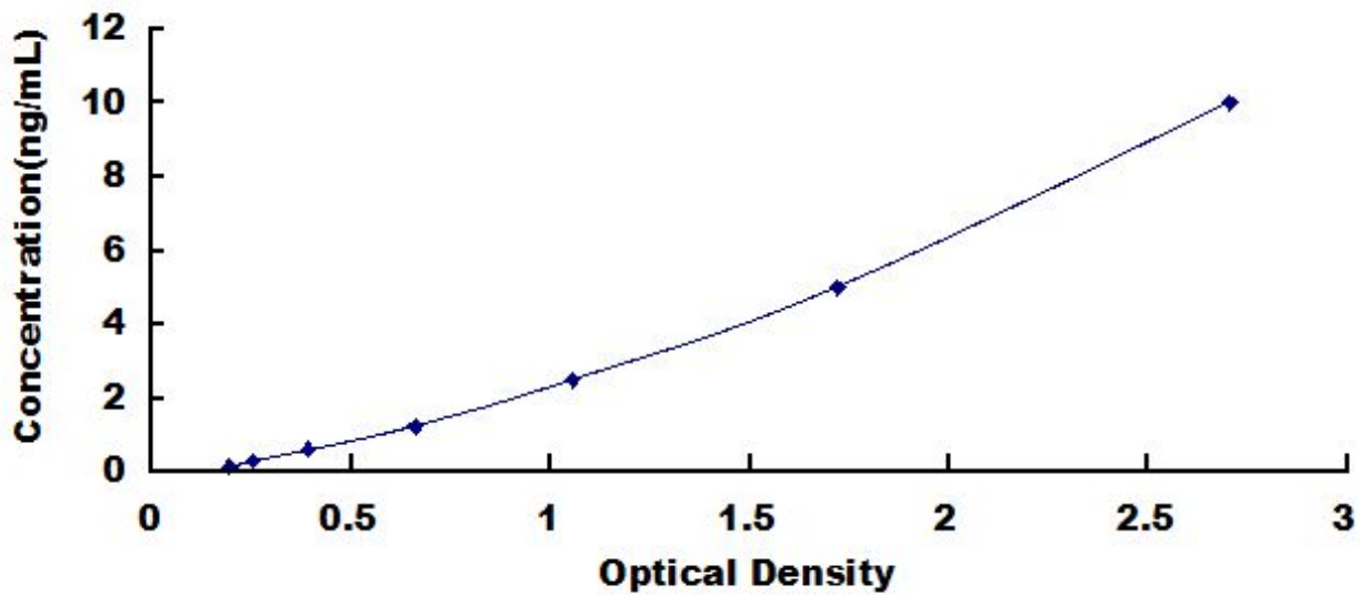
Typical Standard Curve for IGFBP1, Human ELISA.
