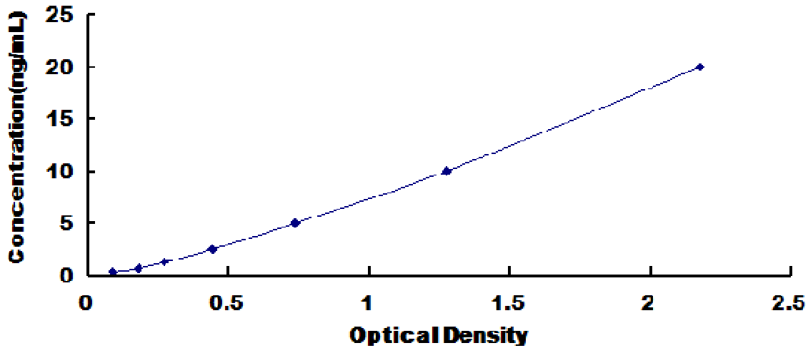
Typical Standard Curve for IAP, Human ELISA.
