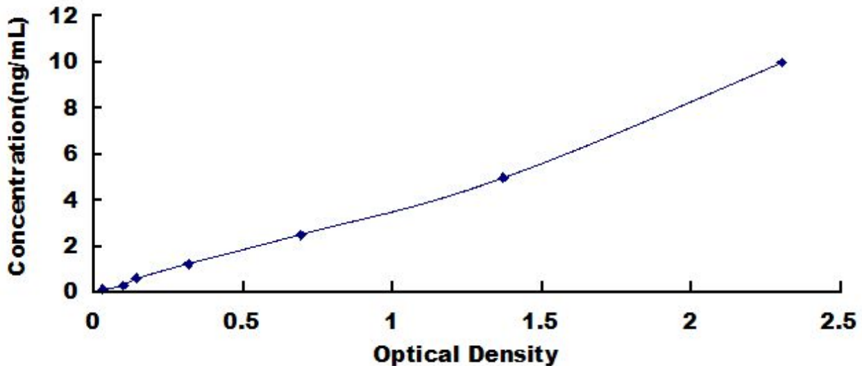
Typical Standard Curve for ITGb6, Human ELISA.
