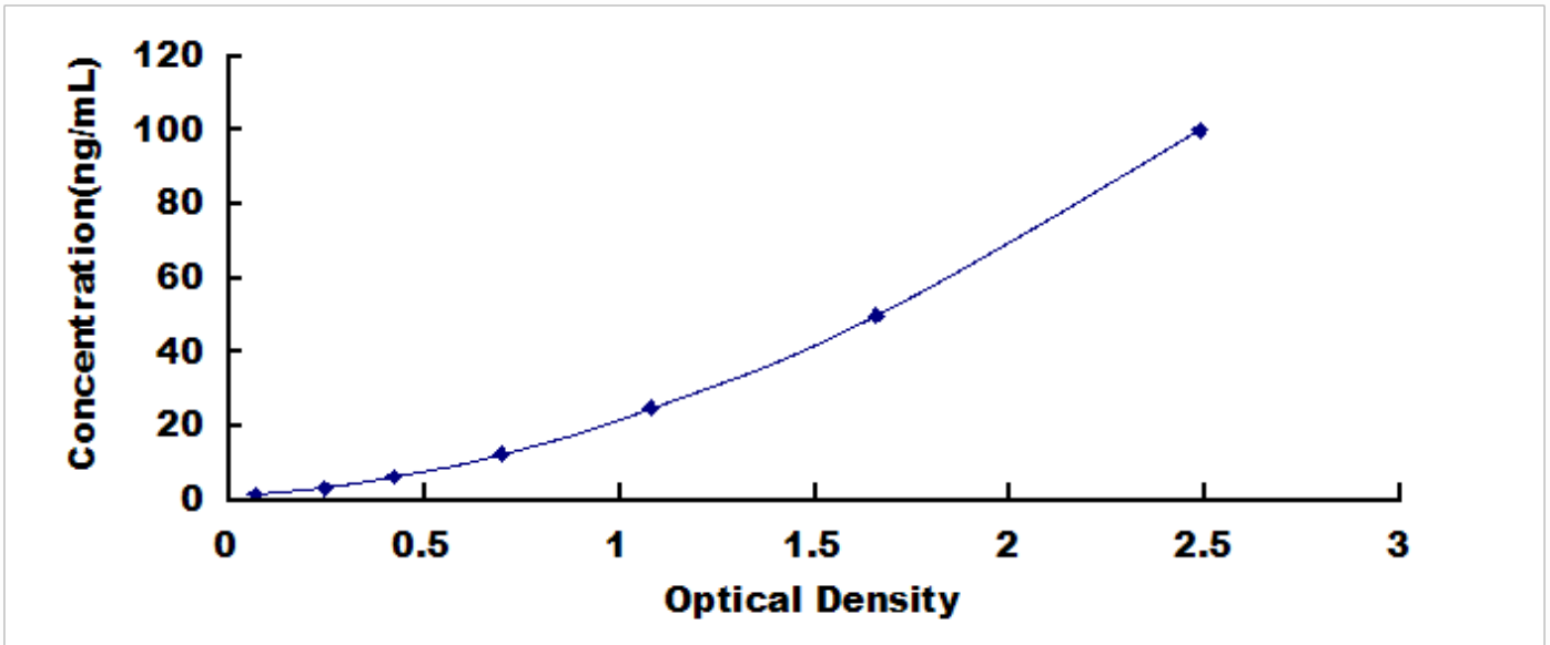
Typical Standard Curve for ICAM1, Porcine ELISA.
