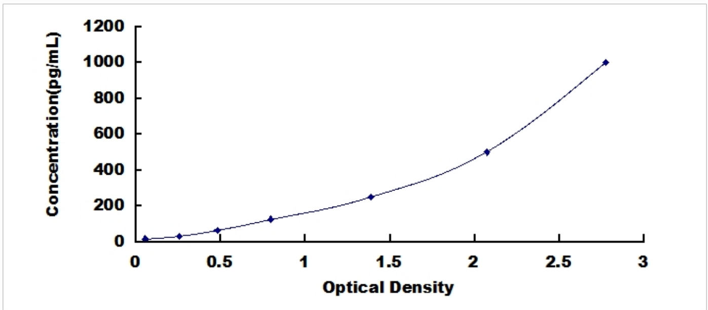
Typical Standard Curve for IFNa, Canine ELISA.
