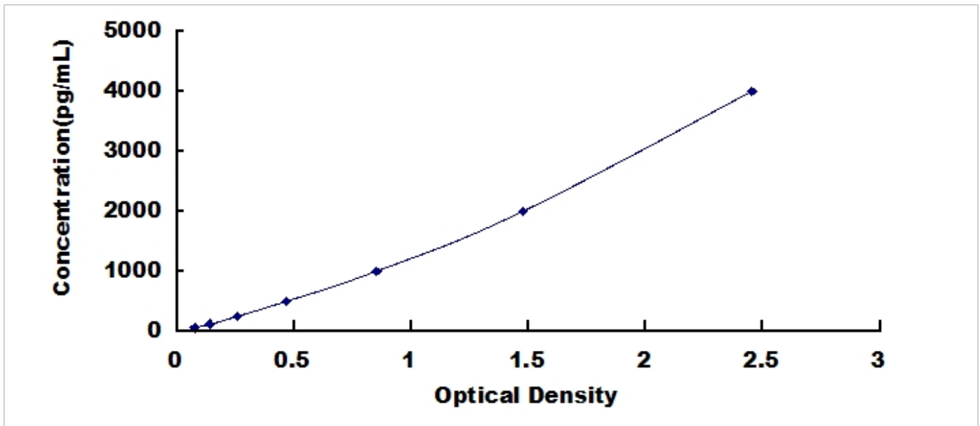
Typical Standard Curve for ITaC, Human ELISA.
