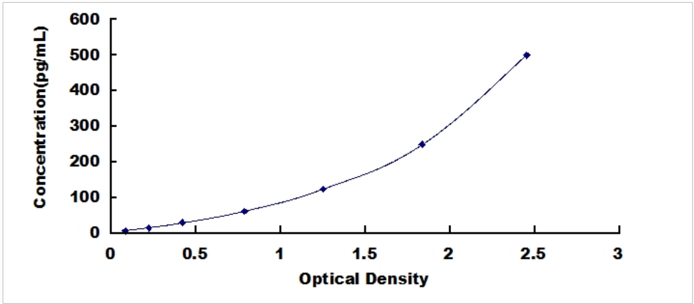
Typical Standard Curve for IL1h, Human ELISA.
