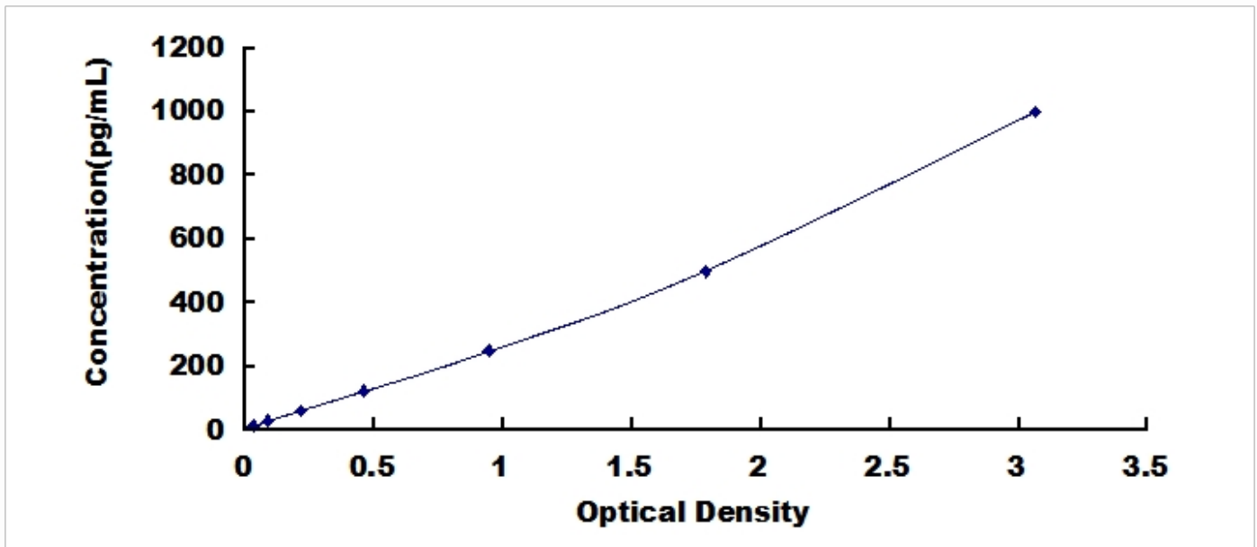
Typical Standard Curve for IL27, Human ELISA.
