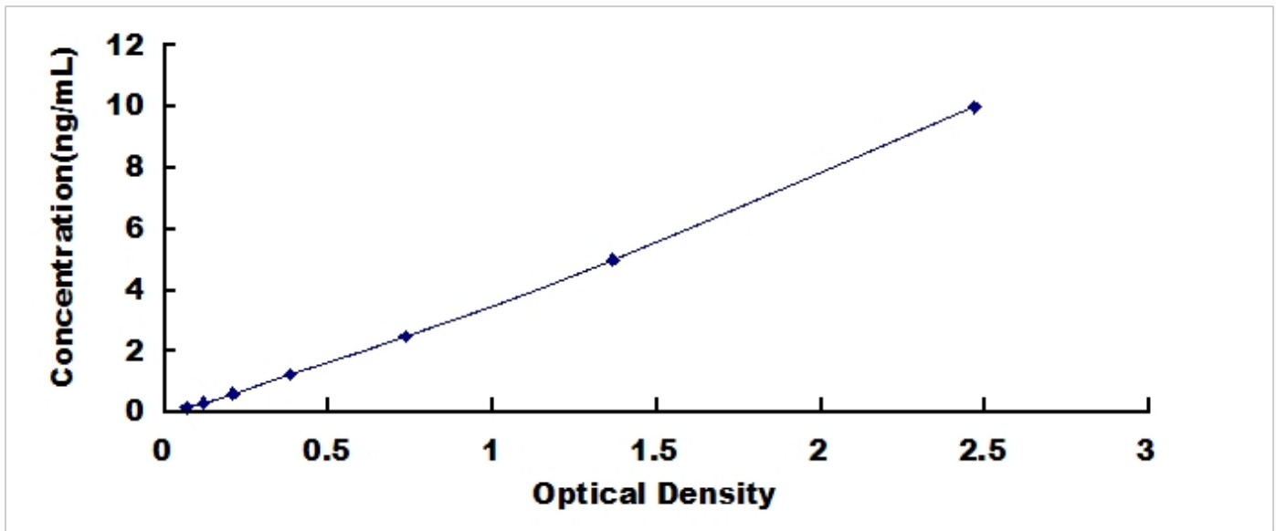
Typical Standard Curve for KLK3, Rat ELISA.
