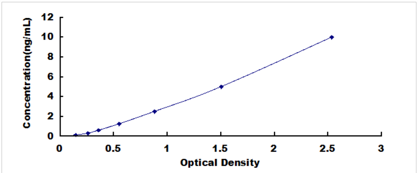
Typical Standard Curve for LSR, Mouse ELISA.
