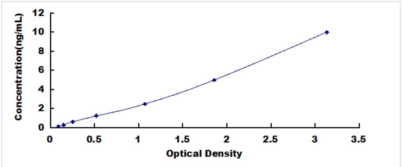
Typical Standard Curve for LEAP2, Human ELISA.
