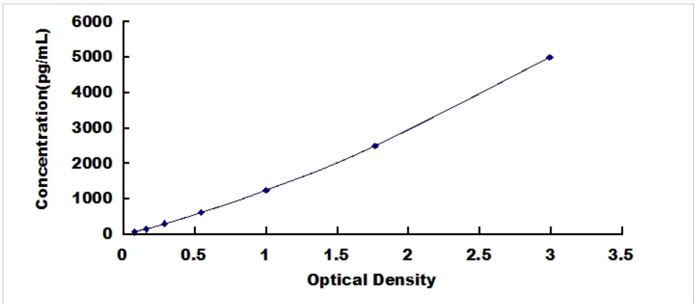
Typical Standard Curve for MTA1, Human ELISA.
