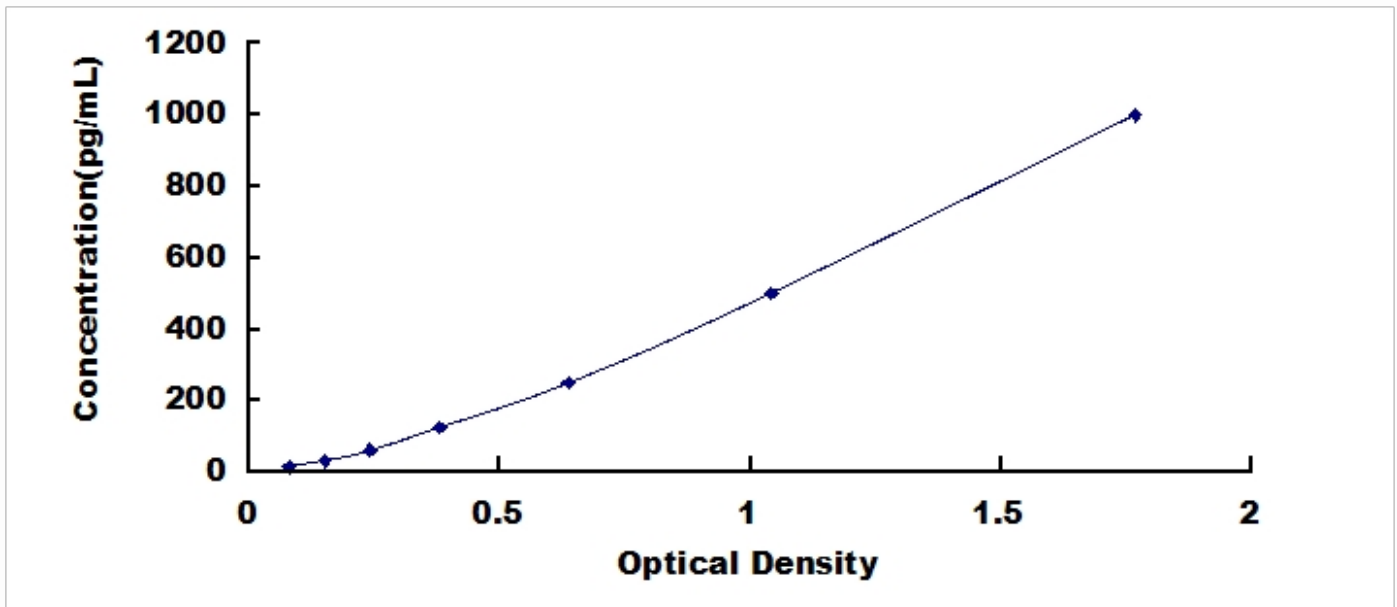
Typical Standard Curve for MCP4, Human ELISA.
