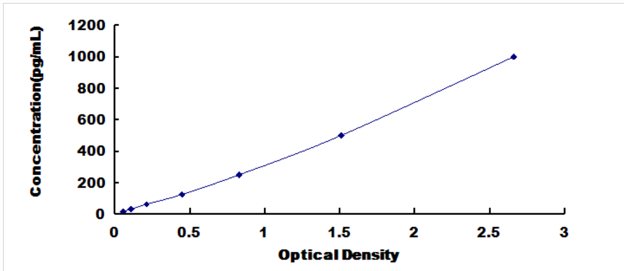
Typical Standard Curve for MUC17, Human ELISA.
