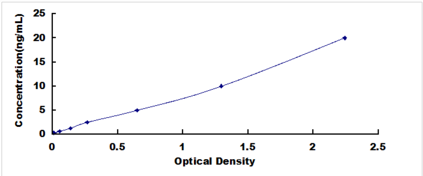
Typical Standard Curve for NRCAM, Mouse ELISA.
