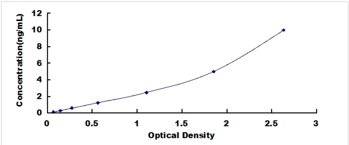
Typical Standard Curve for NTE, Rat ELISA.
