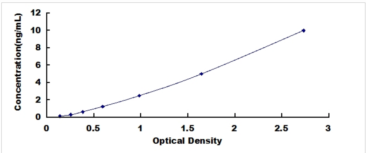
Typical Standard Curve for NUMA1, Human ELISA.
