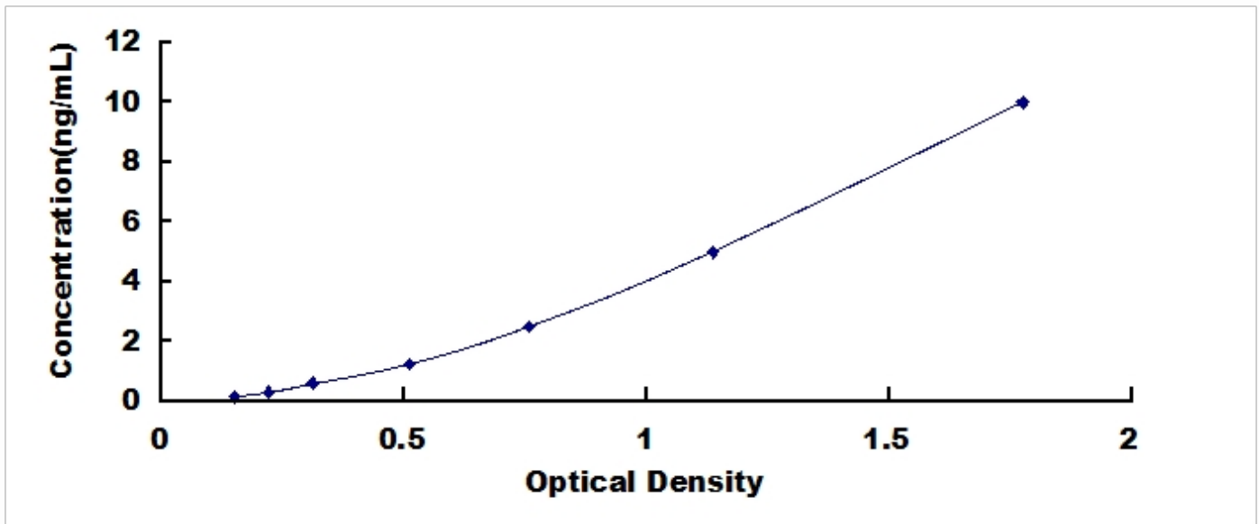
Typical Standard Curve for NUCB1, Human ELISA.
