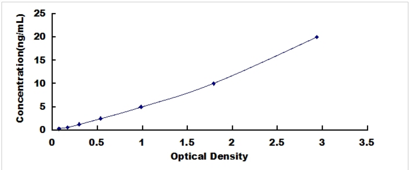
Typical Standard Curve for OGFR, Rat ELISA.
