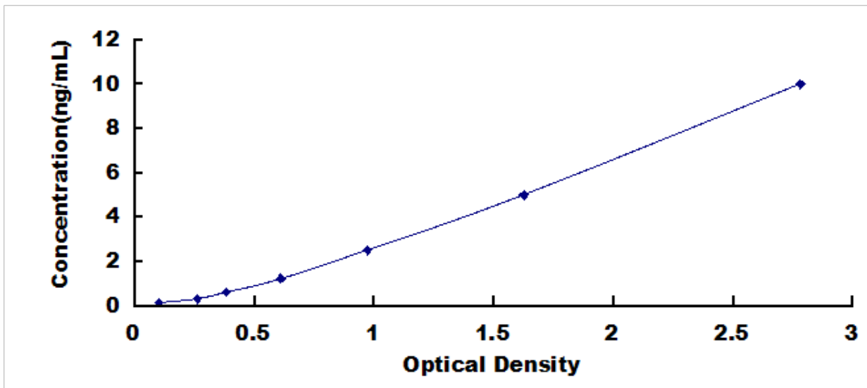
Typical Standard Curve for PGC, Mouse ELISA.
