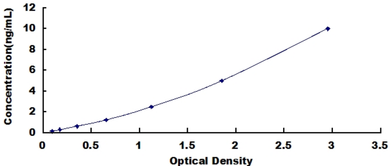
Typical Standard Curve for peripherin, Mouse ELISA.
