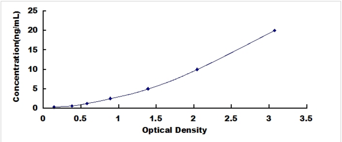
Typical Standard Curve for LpPLA2, Mouse ELISA.
