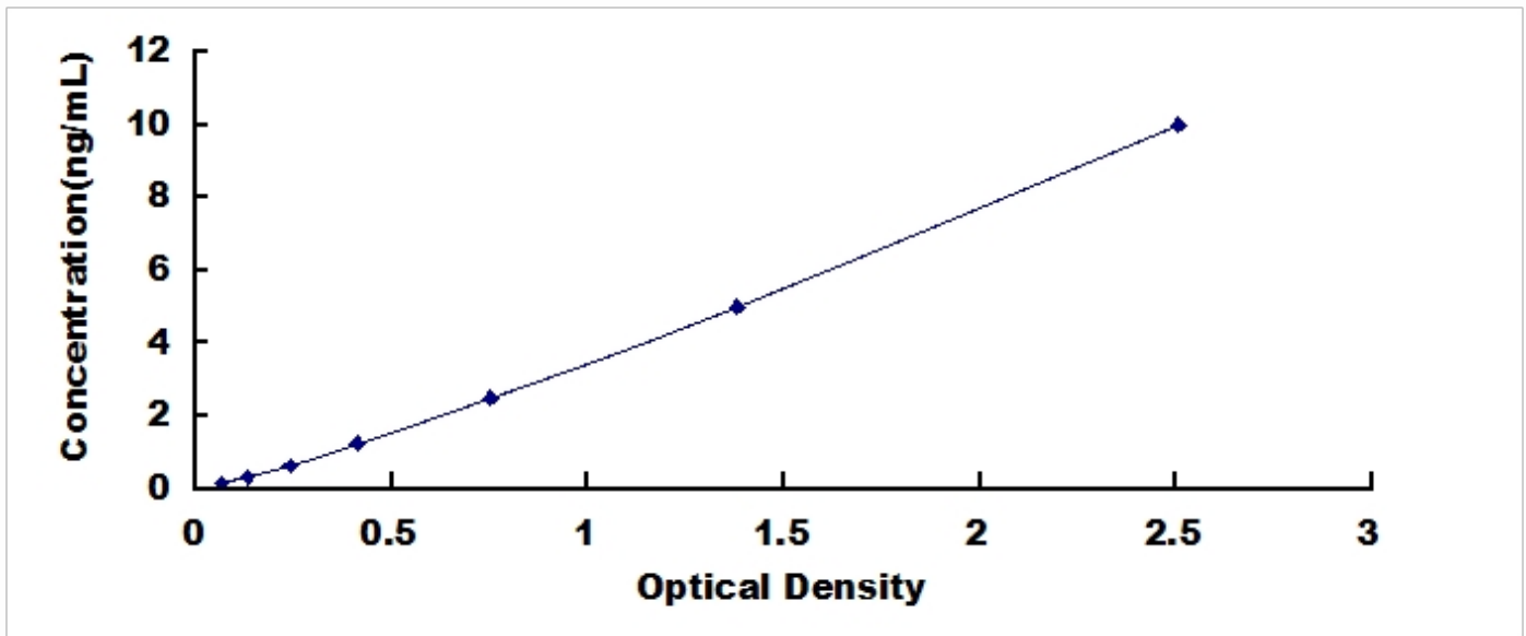
Typical Standard Curve for PFDN2, Human ELISA.
