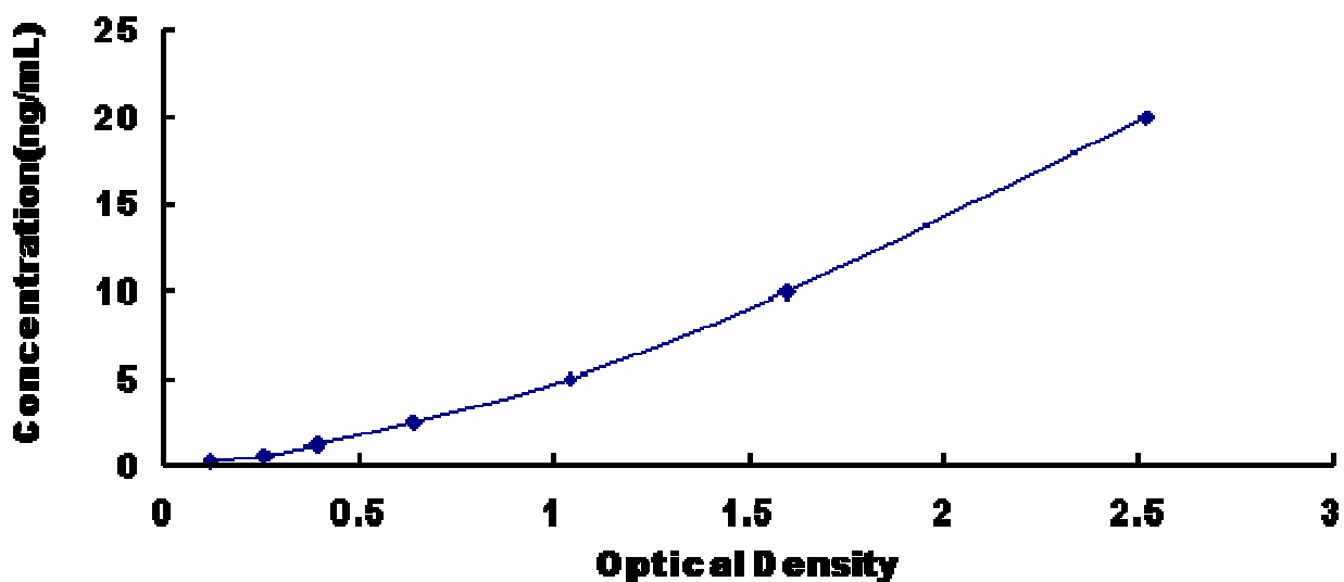
Typical Standard Curve for PDCD6, Human ELISA.
