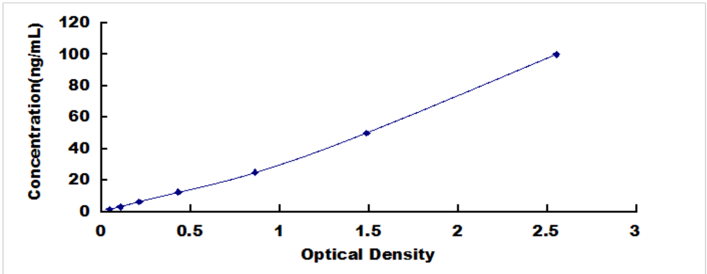
Typical Standard Curve for PDIA4, Human ELISA.
