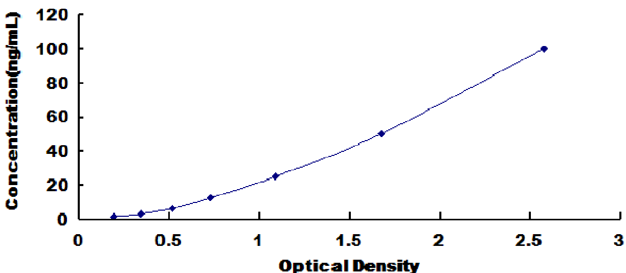
Typical Standard Curve for PC, Human ELISA.
