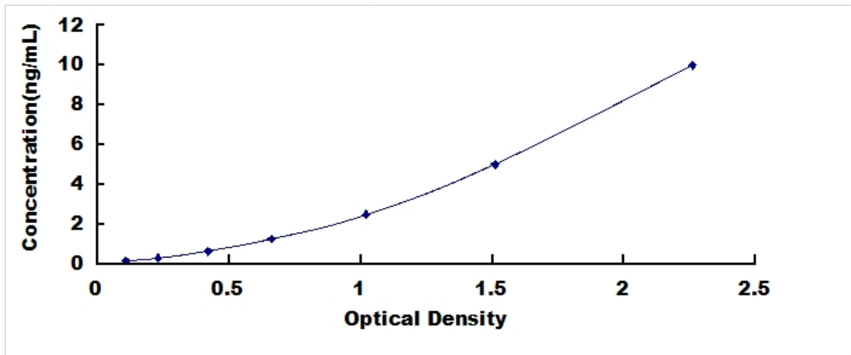
Typical Standard Curve for RGS9, Rat ELISA.
