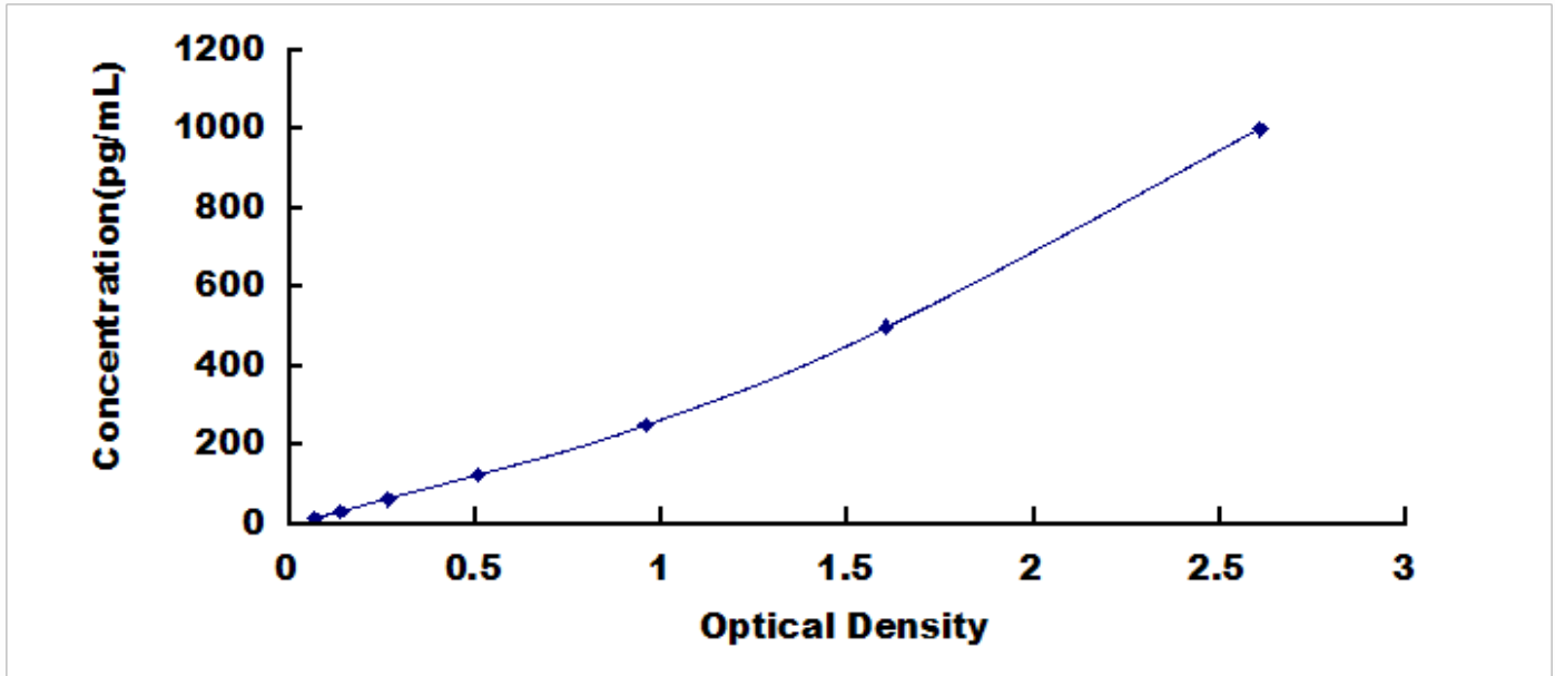
Typical Standard Curve for S100A6, Mouse ELISA.
