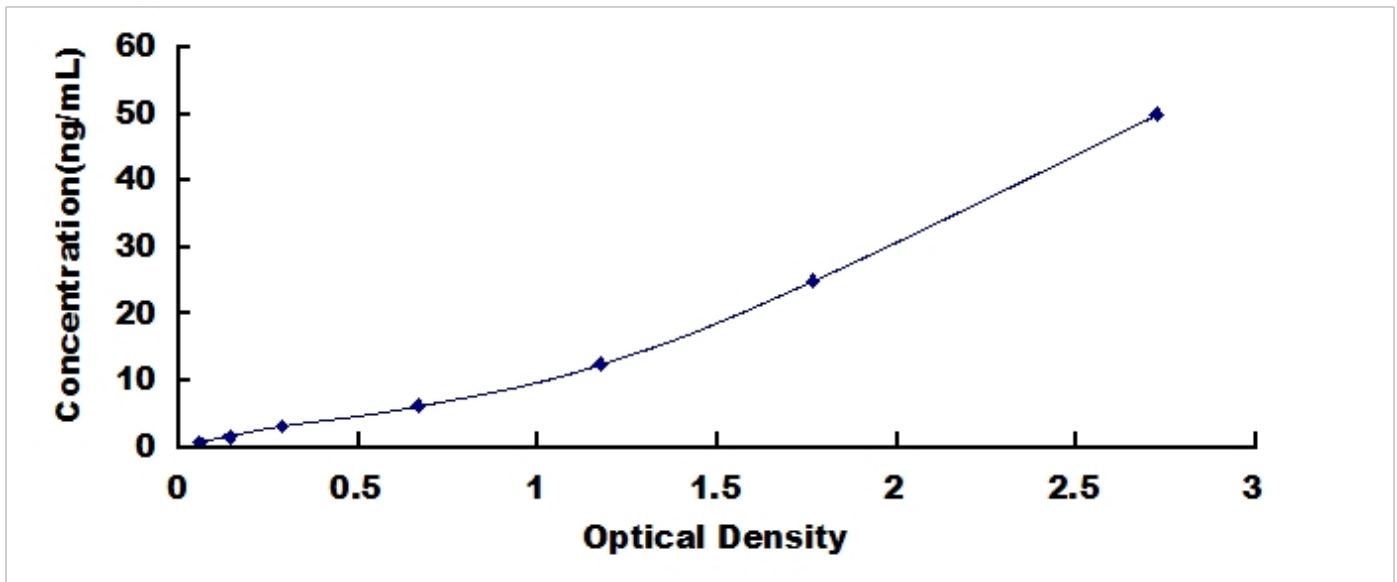
Typical Standard Curve for SECTM1, Human ELISA.
