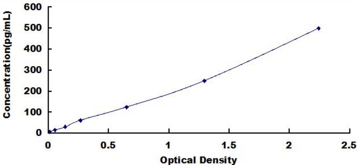
Typical Standard Curve for SCG5, Human ELISA.
