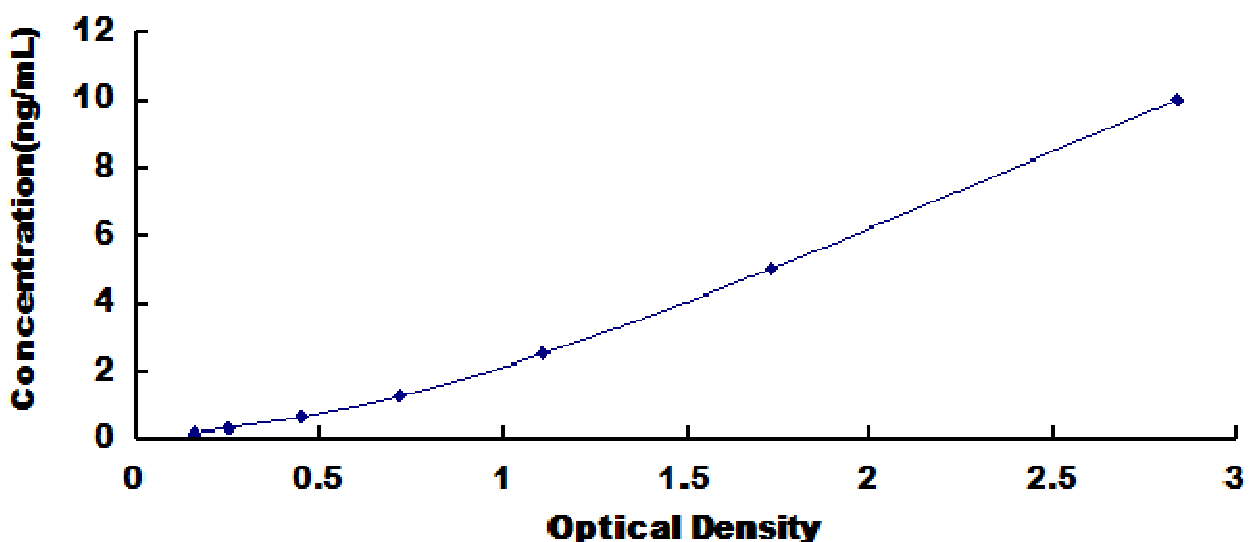
Typical Standard Curve for SGPL1, Mouse ELISA.
