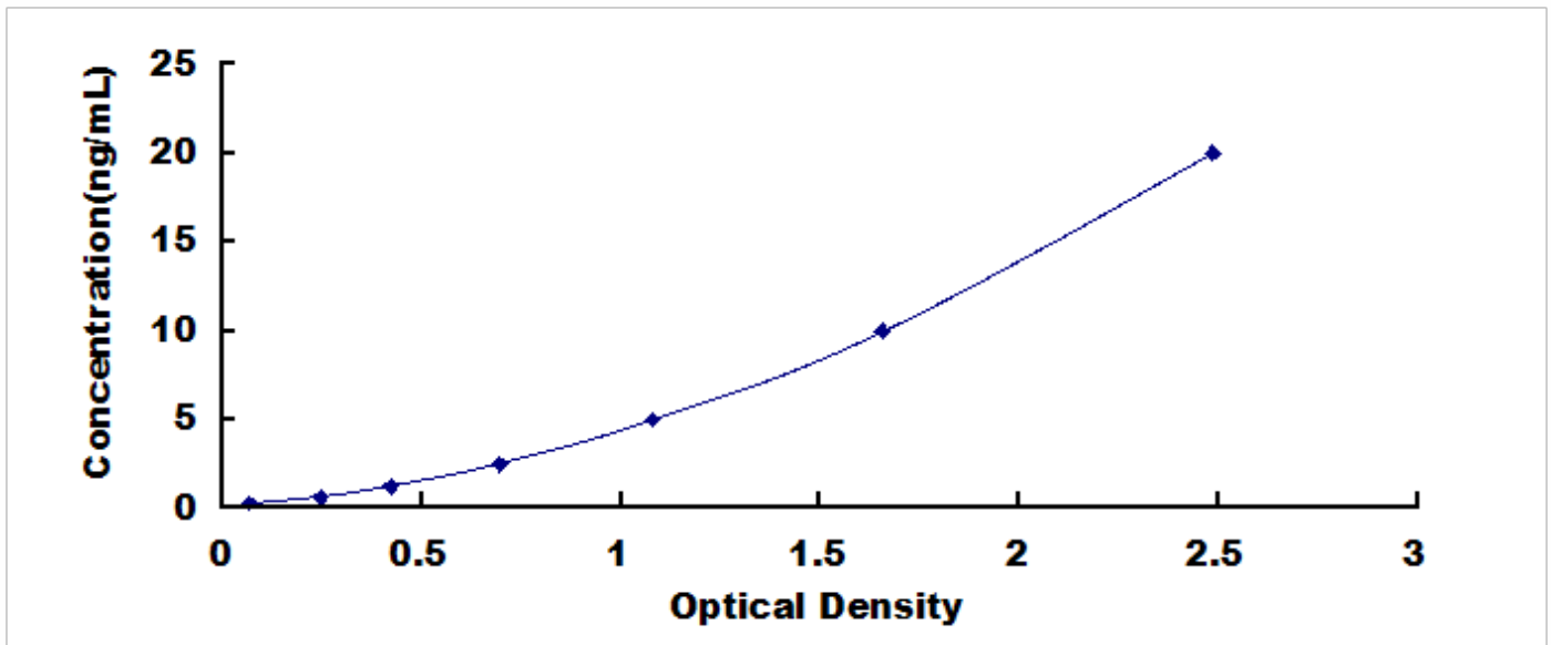
Typical Standard Curve for S1PR2, Mouse ELISA.
