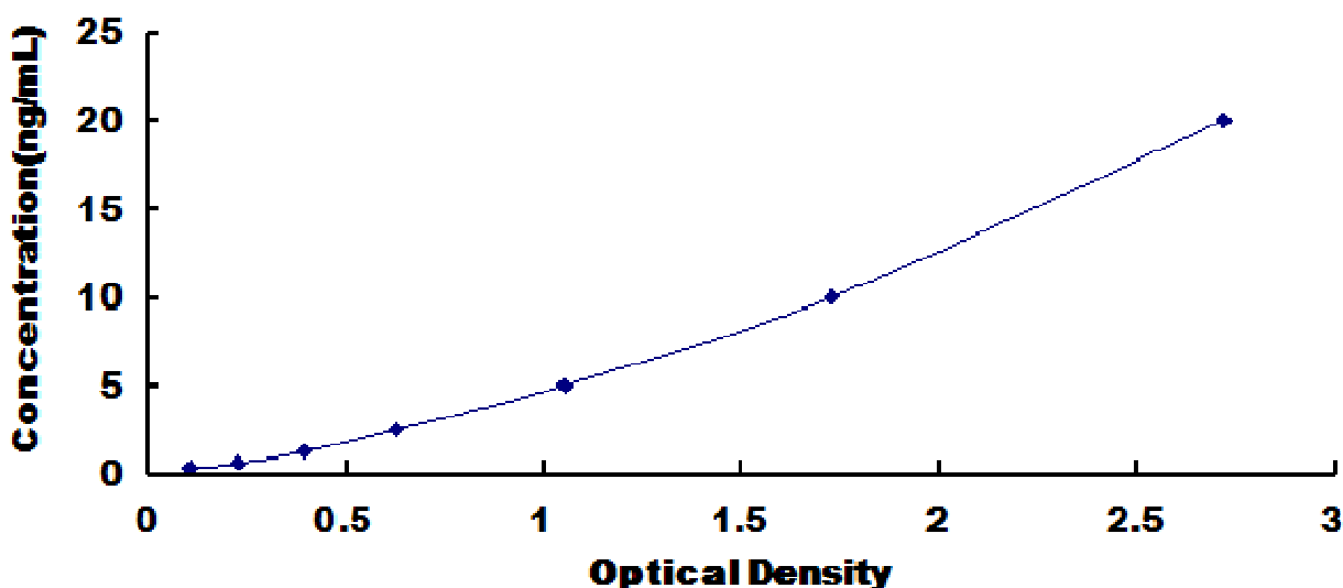
Typical Standard Curve for SOCS2, Rat ELISA.
