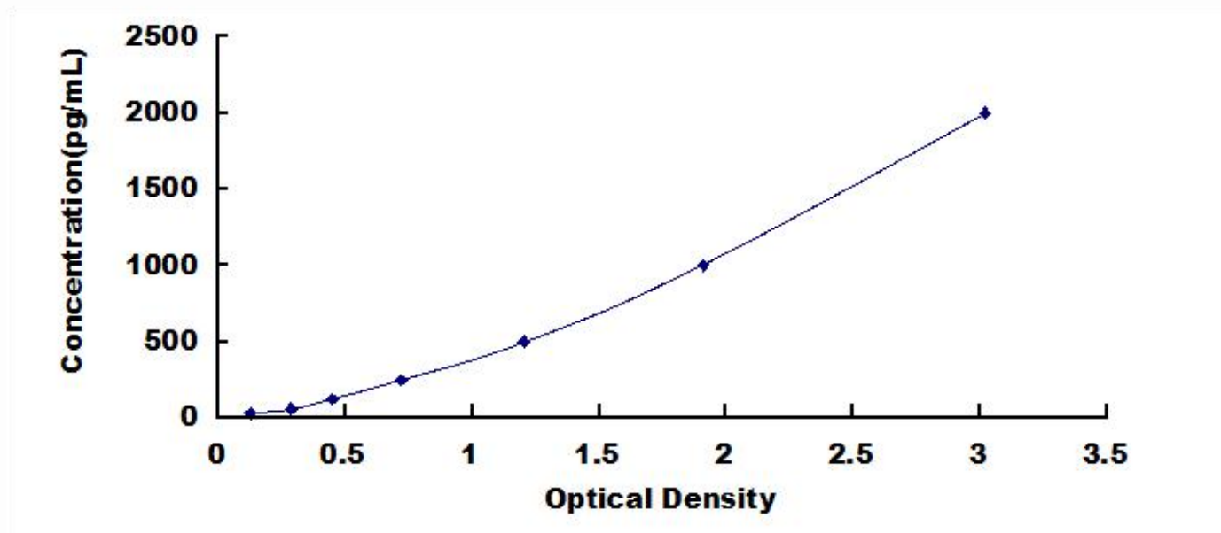
Typical Standard Curve for TNNC1, Human ELISA.
