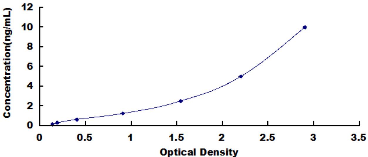
Typical Standard Curve for WARS, Rat ELISA.
