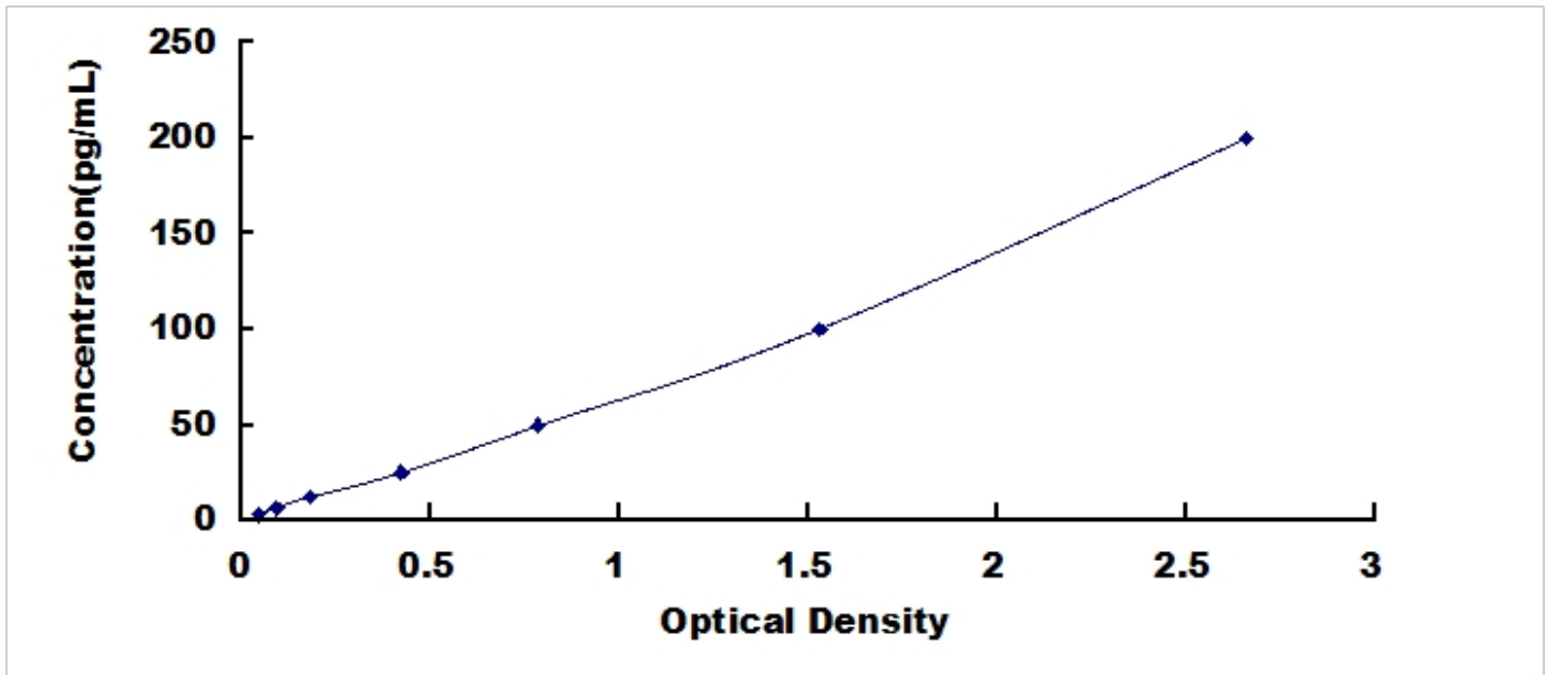
Typical Standard Curve for TNFa, Ovine ELISA.
