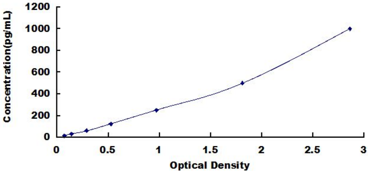
Typical Standard Curve for TNFRSF10B, Human ELISA.
