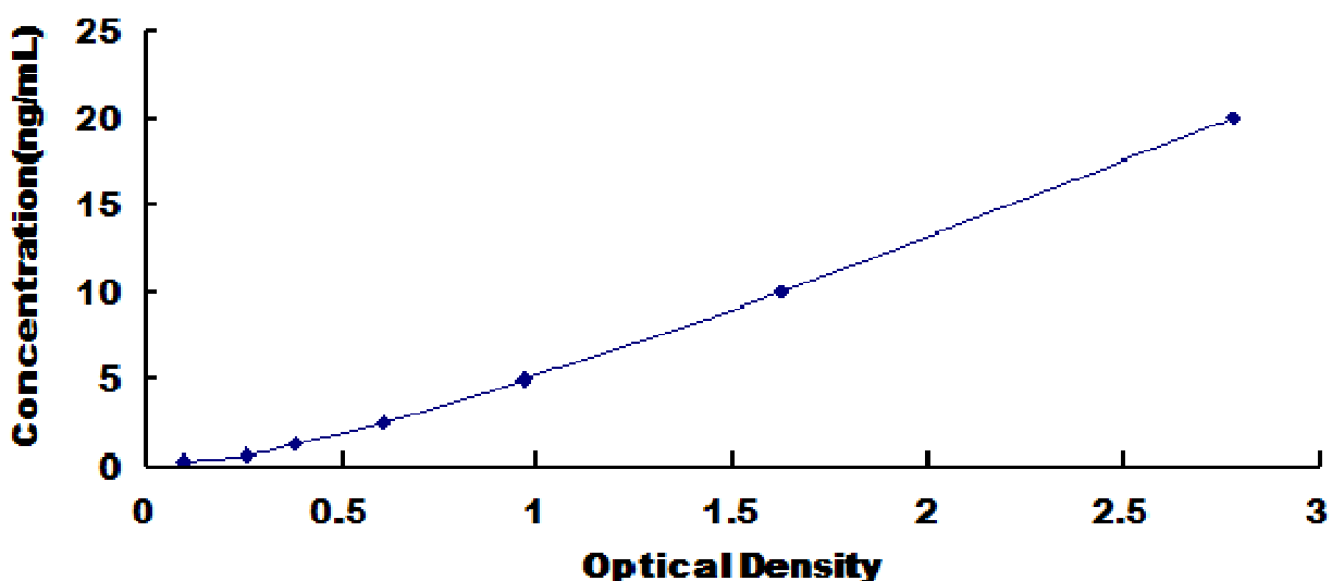
Typical Standard Curve for USP14, Human ELISA.
