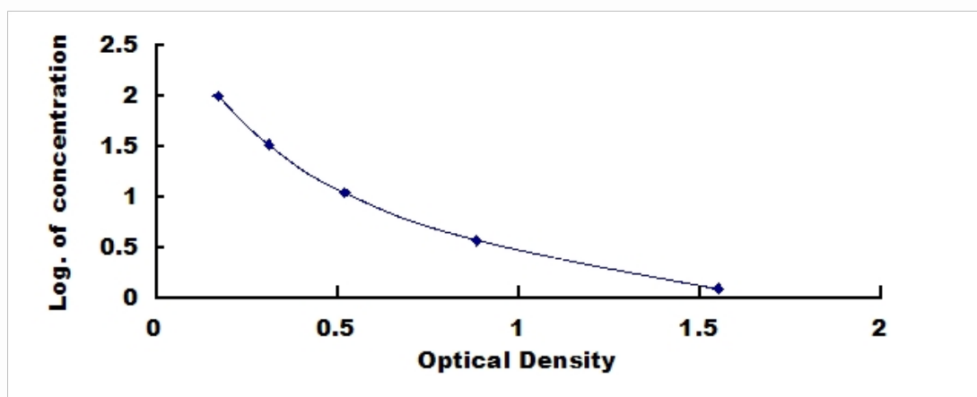
Typical Standard Curve for UCN2, Mouse ELISA.
