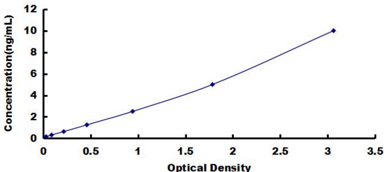
Typical Standard Curve for XBP1, Mouse ELISA.
