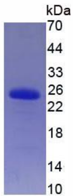
Figure 2. SDS-PAGE
