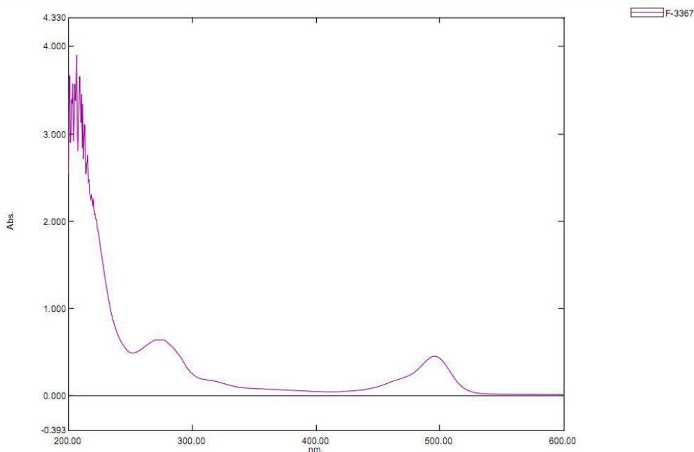
Figure 1: UV-spectrum
