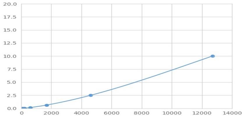
Typical Standard Curve for ACOX1 Magnetic Luminex Assay.
