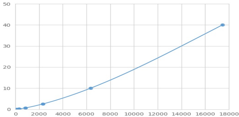
Typical Standard Curve for ABP1 Magnetic Luminex Assay.
